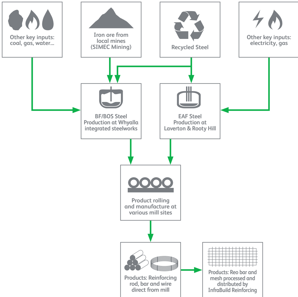
Figure 3: Reinforcing bar and mesh products manufactured by InfraBuild
